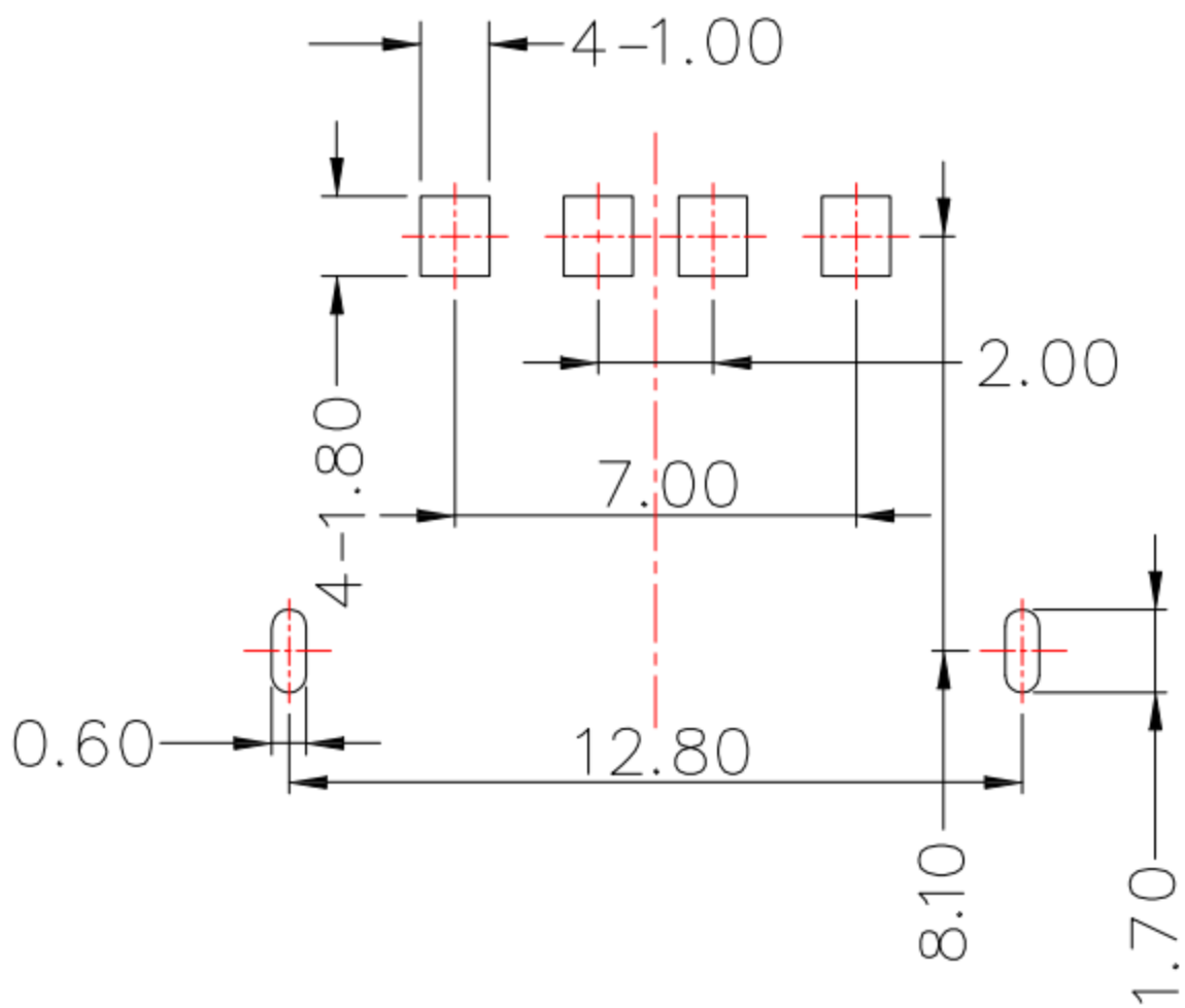
FRONT EDGE OF CONNECTOR PCB LAYOUT
