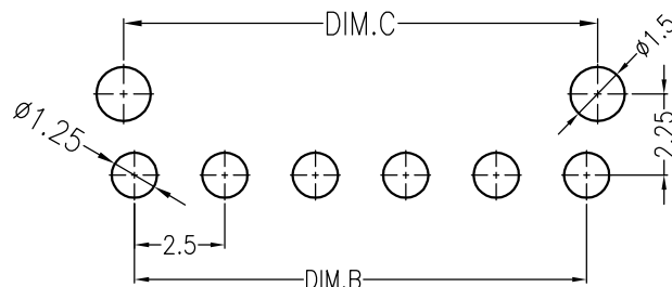
SUGGESTED PCB LAYOUT (COMPONENT SIDE)
