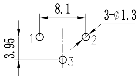
P.C.B LAYOUT (BOTTOM VIEW) Tolerance: \pm 0.05
