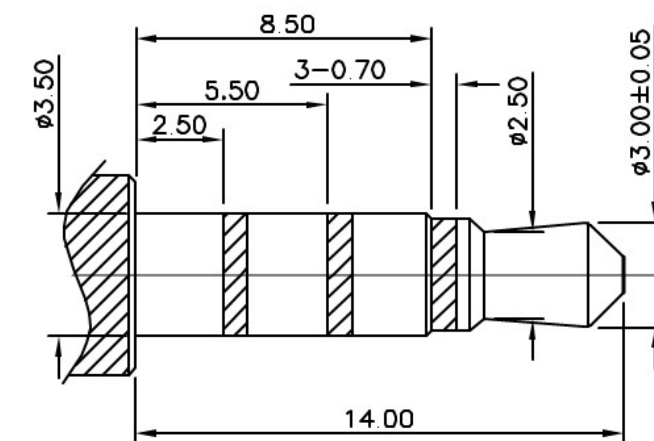
(Ø3.50mm 4 POLE PLUG DETAIL DRAWING)
