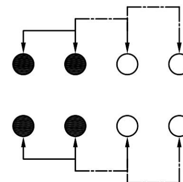
SCHEMATIC (NON-SHORTING)
