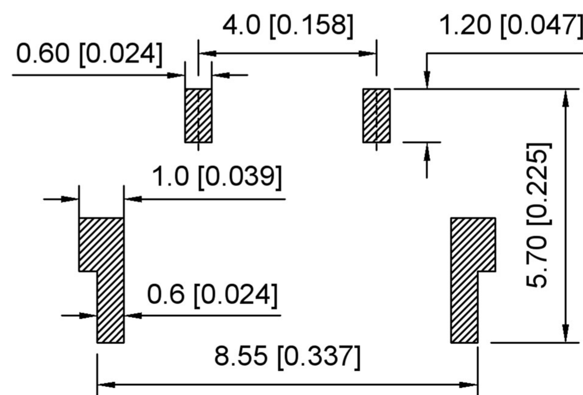
PCB LAYOUT
