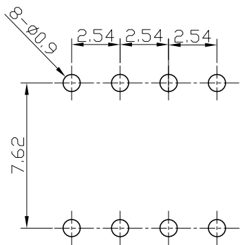
P. C. B LAYOUT
