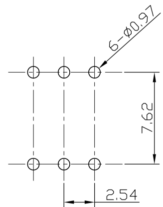
P. C. B LAYOUT
