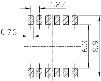
P. C. B LAYOUT
